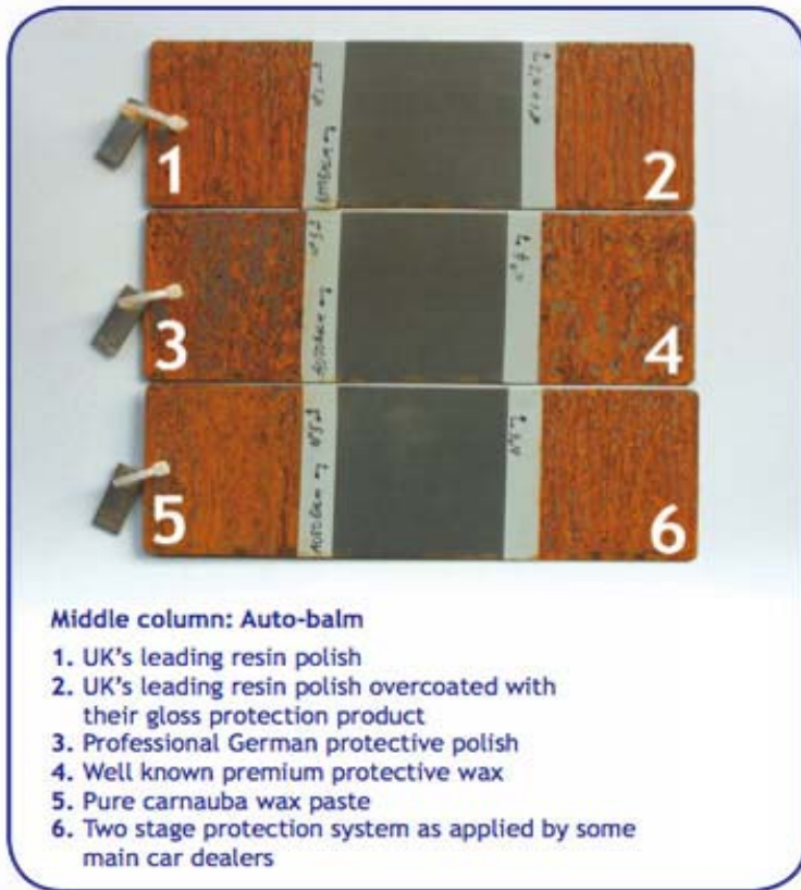
Test Panels - after 24 hours in hot salt spray cabinet
